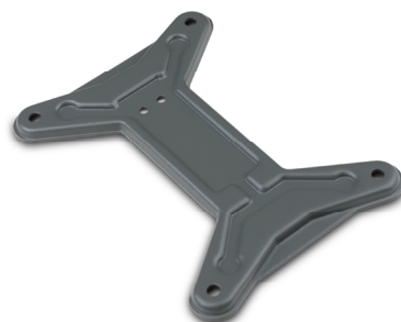
Full-pressed steel base Designed to withstand rough condition using full-pressed steel for scale base & loadcell mounting.
